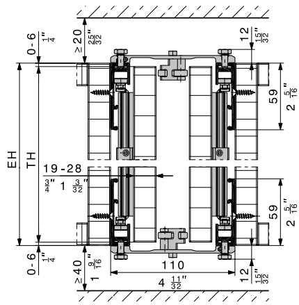
System: Hawa Concepta 25/30 Connection: Connector 110 mm (4 11/32")
