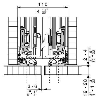
Connector 110 mm (4 11/32") Maximum door thickness: 28 mm (1 1/16")
