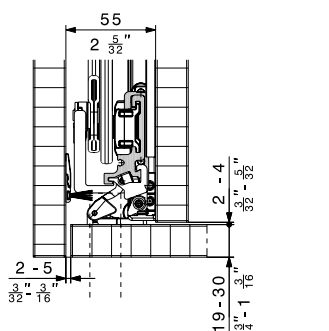
Connector 55 mm (2 3/32") Maximum door thickness: 30 mm (1 1/8")
