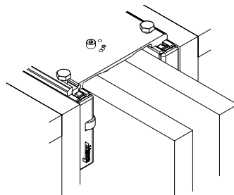
Connector 110 mm (4 11 / 32 " ): recess for two pivot/slide-in doors
