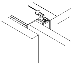
Connector 55 mm (2 3 / 16 " ): recess for one pivot/slide-in door
