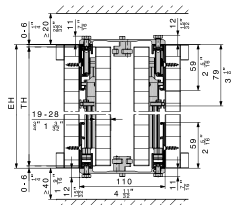
System: Hawa Concepta 40/50 Connection: Connector 110 mm (4 11/32")
