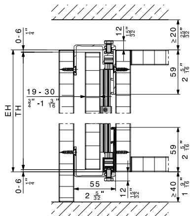
System: Hawa Concepta 25/30 Connection: Connector 55 mm (2 3/32")
