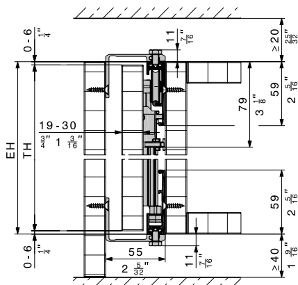
System: Hawa Concepta 40/50 Connection: Connector 55 mm (2 3/32")
